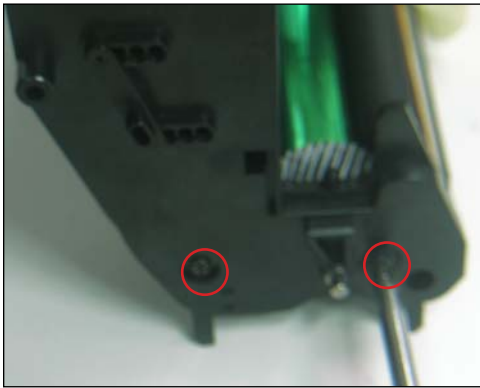
9. Remove the two screws that hold the end cap (gearless) in place as shown.
