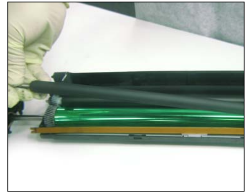
11. The PCR can now be removed as shown.
