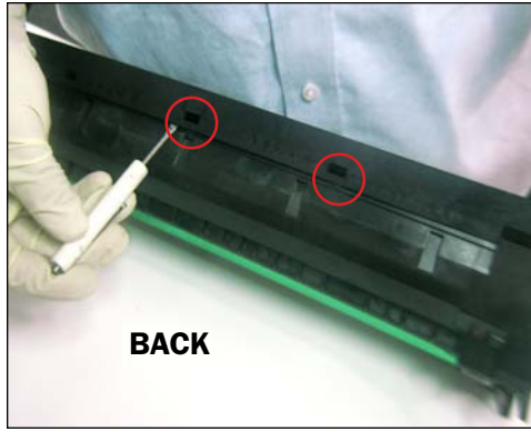
5. Use a small flathead screwdriver to push in the five tabs located on the back and front of the cartridge to unlock the drum unit cover.
