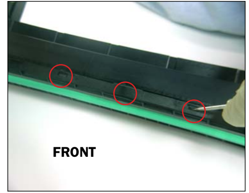
5. Use a small flathead screwdriver to push in the five tabs located on the back and front of the cartridge to unlock the drum unit cover.
