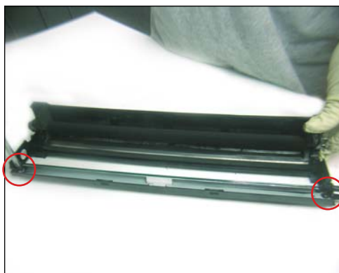
18. Remove the two screws on both ends of the wiper blade that hold it in place.
