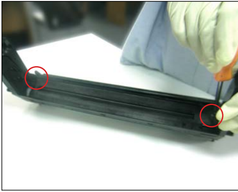
4. Remove the two screws located on the the top of the drum unit cover that hold it in place.
