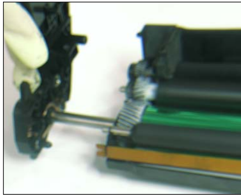
10. Slide the the end cap out by approximately. two inches. The drum axle is connected to it.
