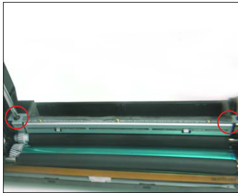
7. Remove the two screws that hold the doctor blade in place as shown.
